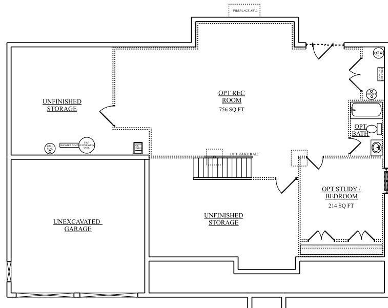
LOWER LEVEL 1818 SQ FT
