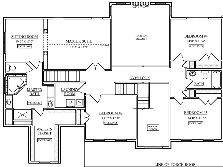
UPPER LEVEL 1678 SQ FT
