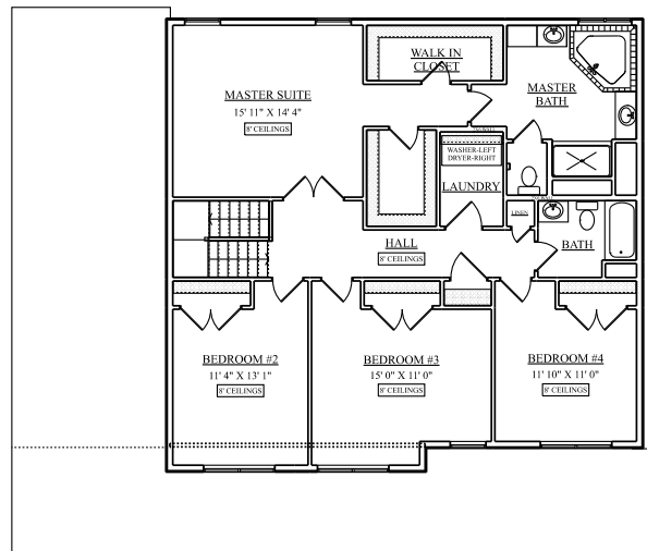
UPPER LEVEL 1426 SQ FT
