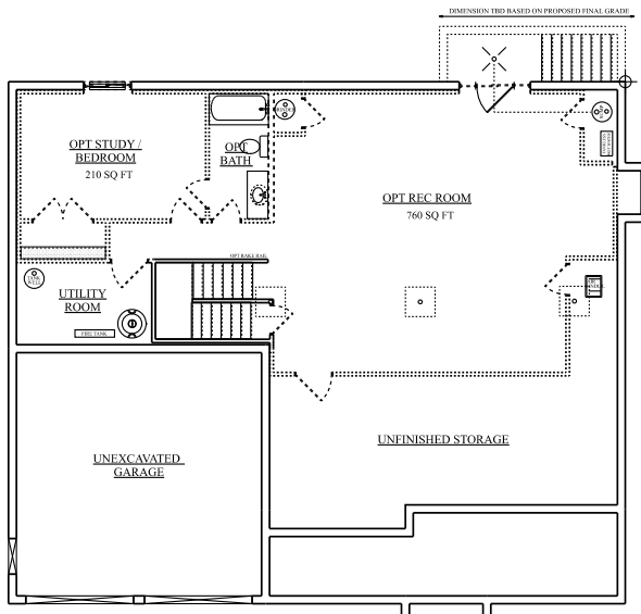
LOWER LEVEL 1637 SQ FT
